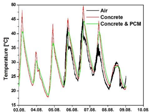
Fig. 6: Temperature profile of concrete tiles with and without PCM inside left outside in the sun.
