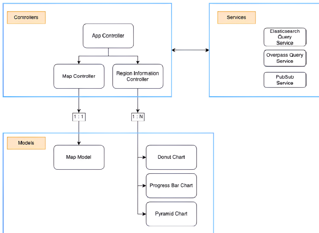
Fig. 3: MVC Design
