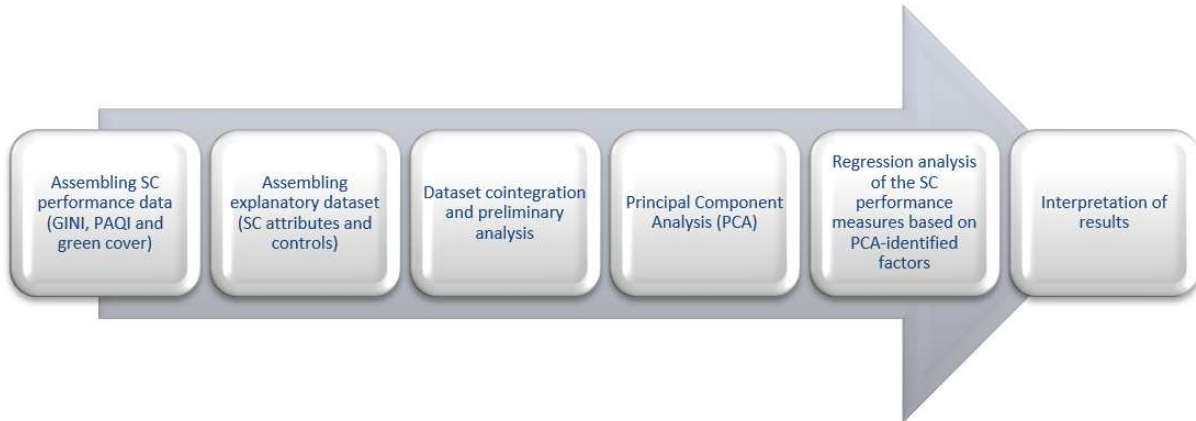
Fig. 2: Study flowchart
