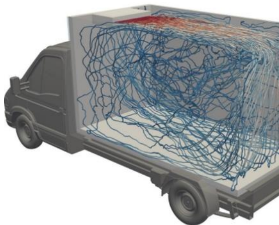
Fig. 9: Simulated flow elements within a delivery truck.
